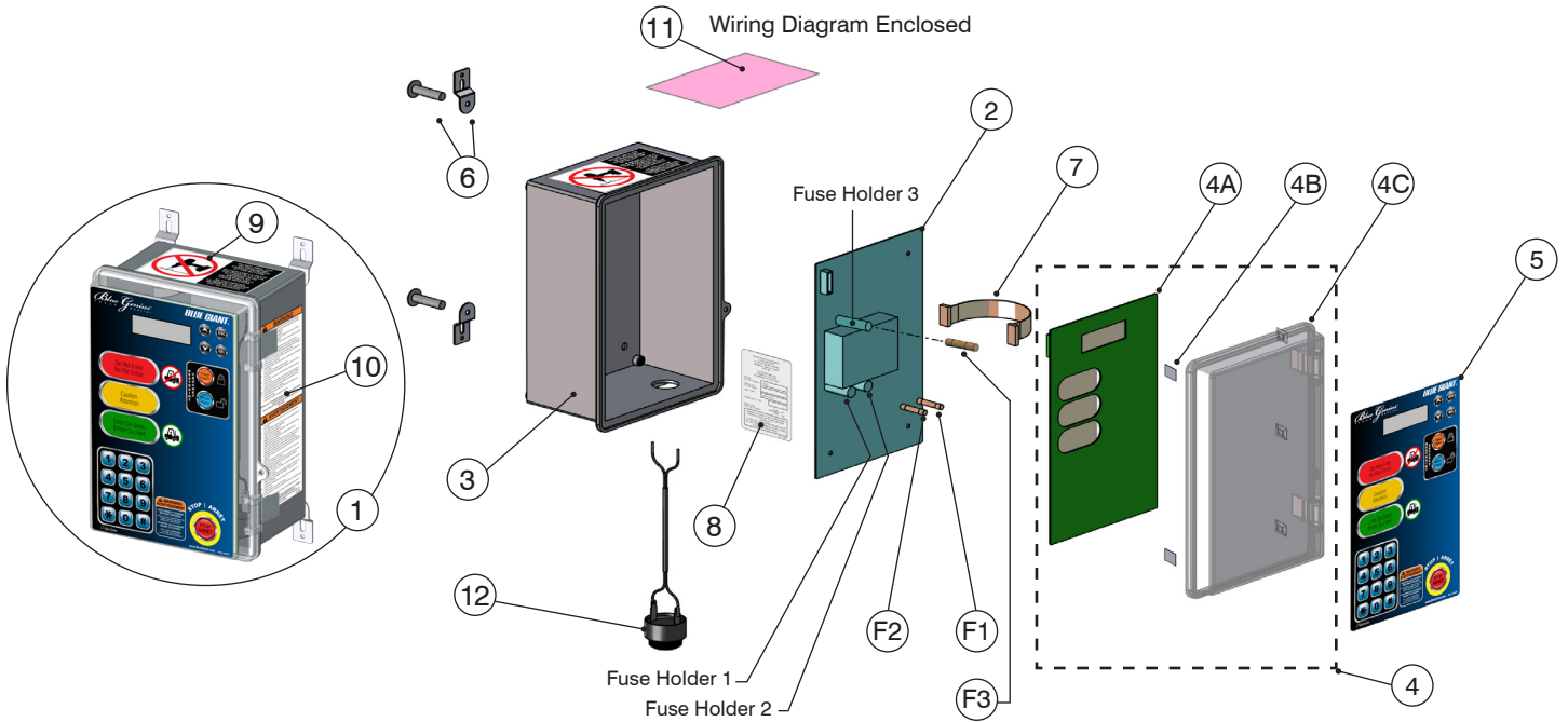
COMPLETE CONTROL STATION ASSEMBLY - ITEM 1 (Example BGGFS1115F)
